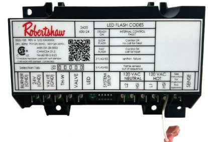
780U-HS30 HOT SURFACE IGNITION
