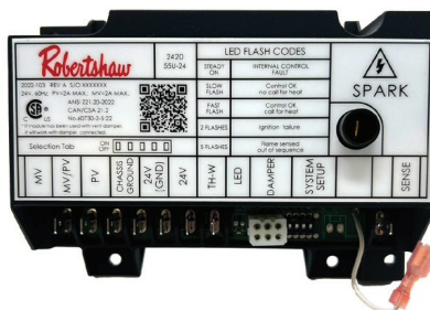
780U-IP10 INTERMITTENT PILOT
